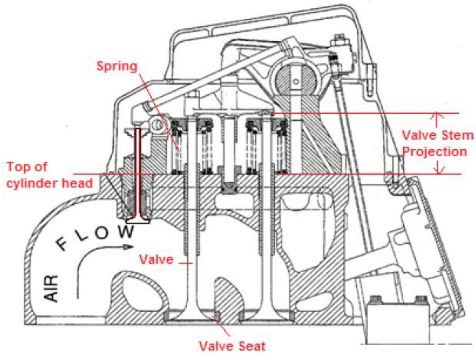
Figure 7: Valve stem projection measurement.
