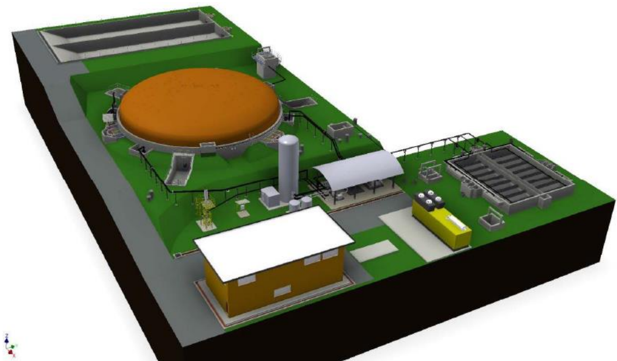
Figure 25: Jeng Huat Kemayan project: Site overview.
