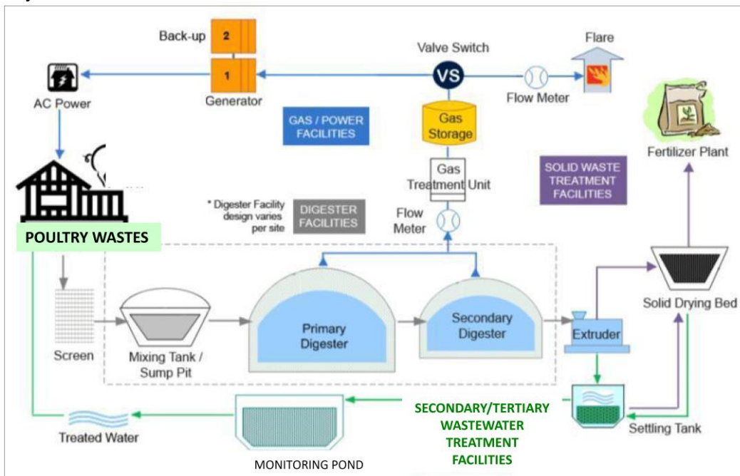
Figure 19: Anaergia SCCF Singapore project: Process flow diagram.
