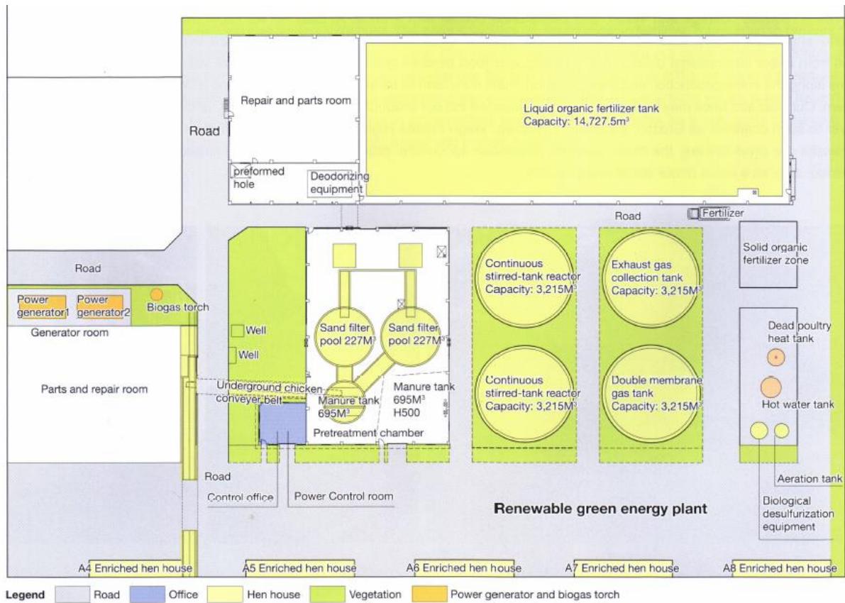
Figure 13: ShiAn Tainan Project: Plant layout.
