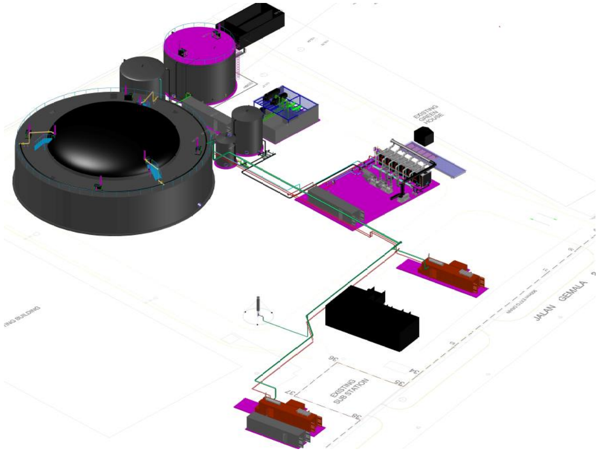
Figure 20: Anaergia SCCF Singapore project: Plant layout diagram.
