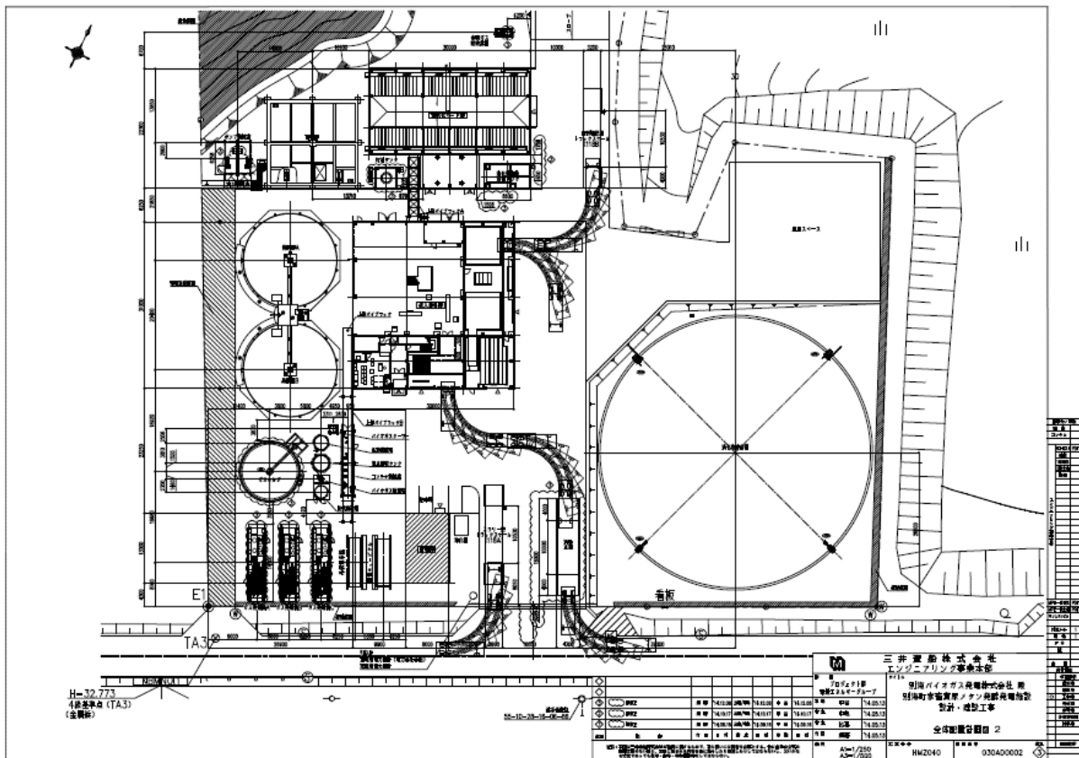
Figure 5: MES Hokkaido biogas-to-power project: Basic layout.
